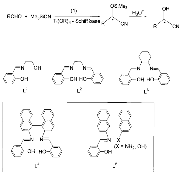
Scheme 1 Asymmetric trimethylsilylcyanation of aldehydes with Me 3 SiCN catalysed by titanium Schiff base complexes. The types of Schiff bases which have been extensively studied (L 1 –L 3 ) are indicated. The inset shows the main types of Schiff bases involved in this work (L 4 and L 5 ).
