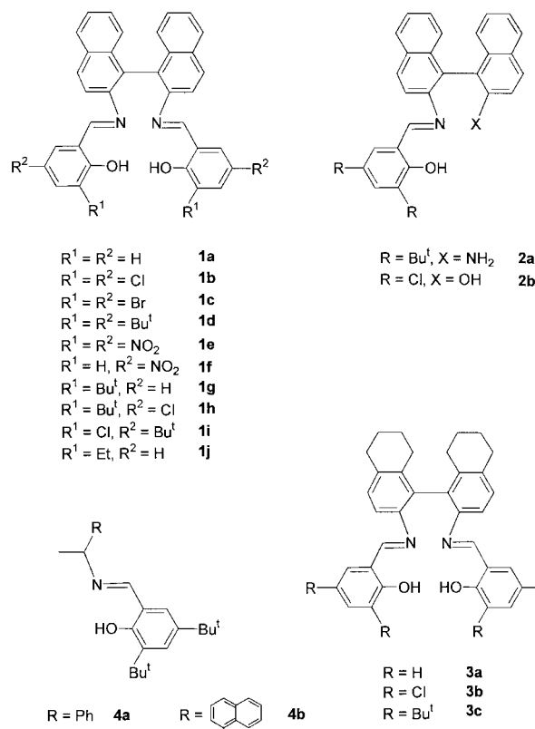
Scheme 1 Asymmetric trimethylsilylcyanation of aldehydes with Me 3 SiCN catalysed by titanium Schiff base complexes. The types of Schiff bases which have been extensively studied (L 1 –L 3 ) are indicated. The inset shows the main types of Schiff bases involved in this work (L 4 and L 5 ).
